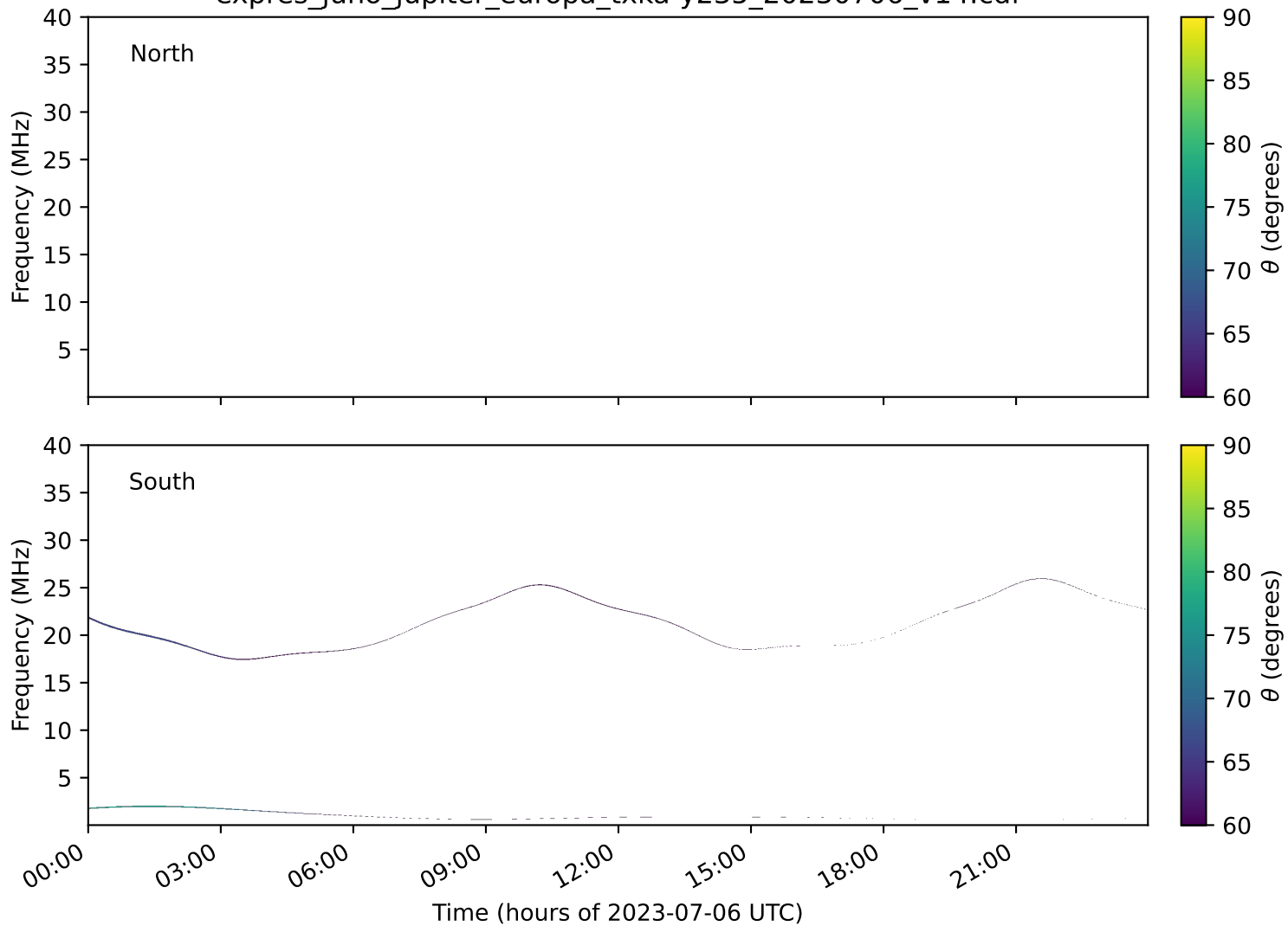
expres_juno_jupiter_europa_txka-y235_20230706_v14.cdf
