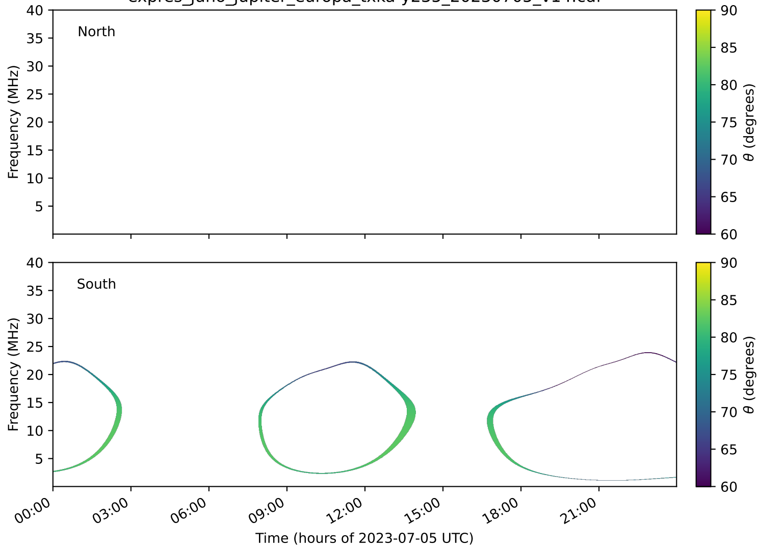
expres_juno_jupiter_europa_txka-y235_20230705_v14.cdf
