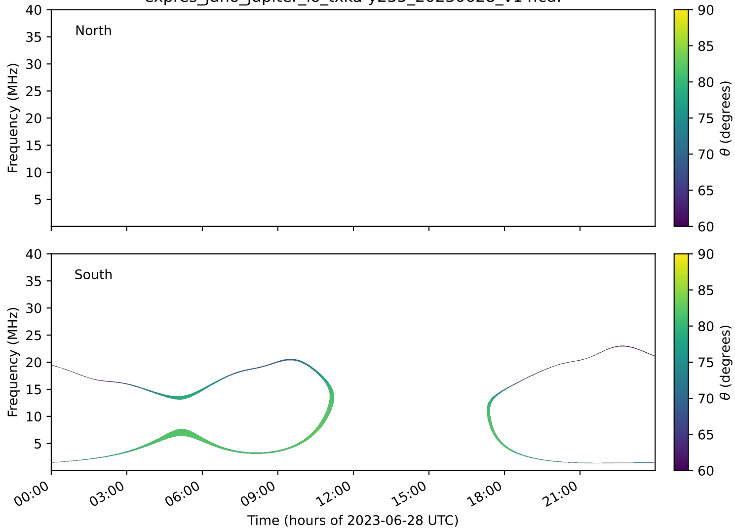
expres_juno_jupiter_io_txka-y235_20230628_v14.cdf
