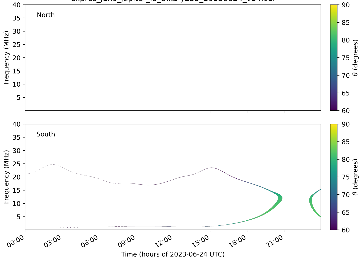
expres_juno_jupiter_io_txka-y235_20230624_v14.cdf
