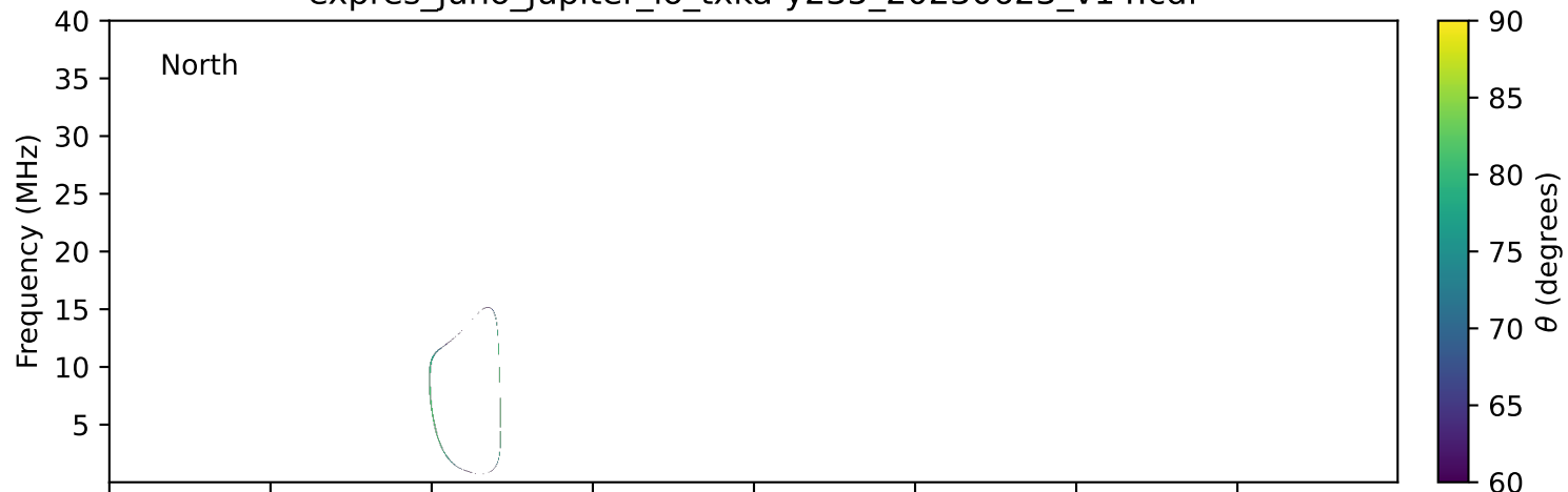
expres_juno_jupiter_io_txka-y235_20230623_v14.cdf
