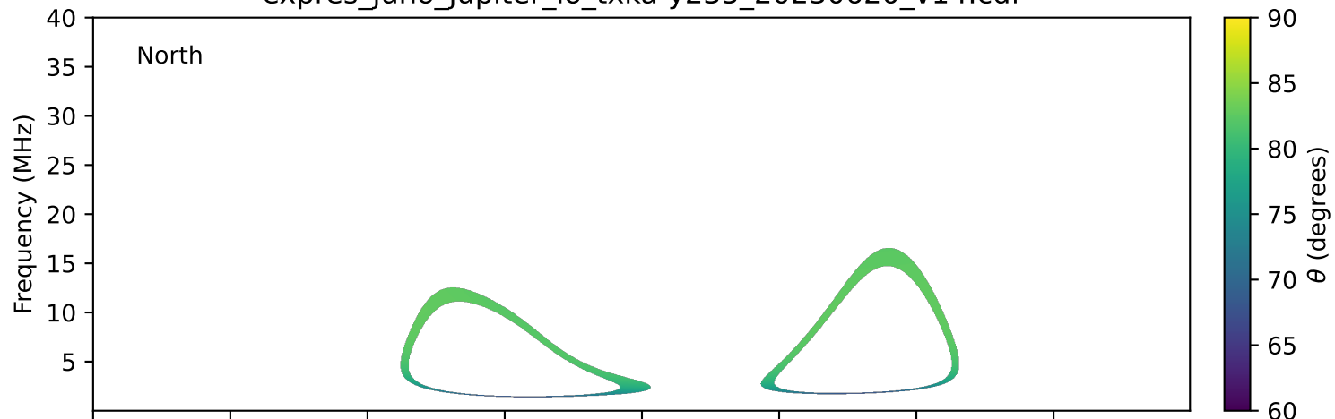
expres_juno_jupiter_io_txka-y235_20230620_v14.cdf
