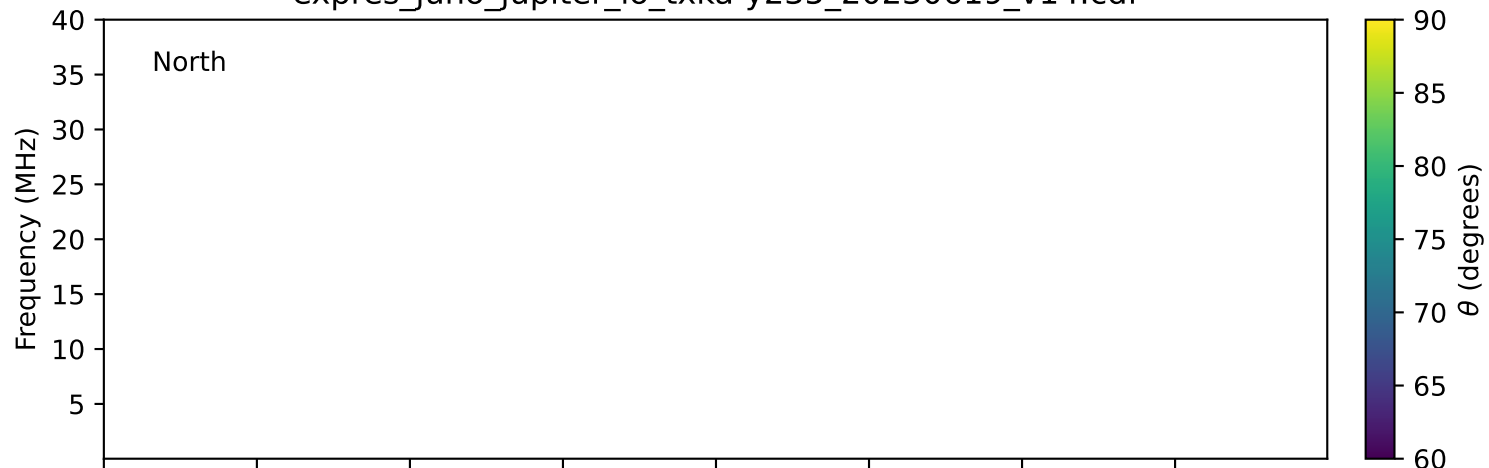
expres_juno_jupiter_io_txka-y235_20230619_v14.cdf
