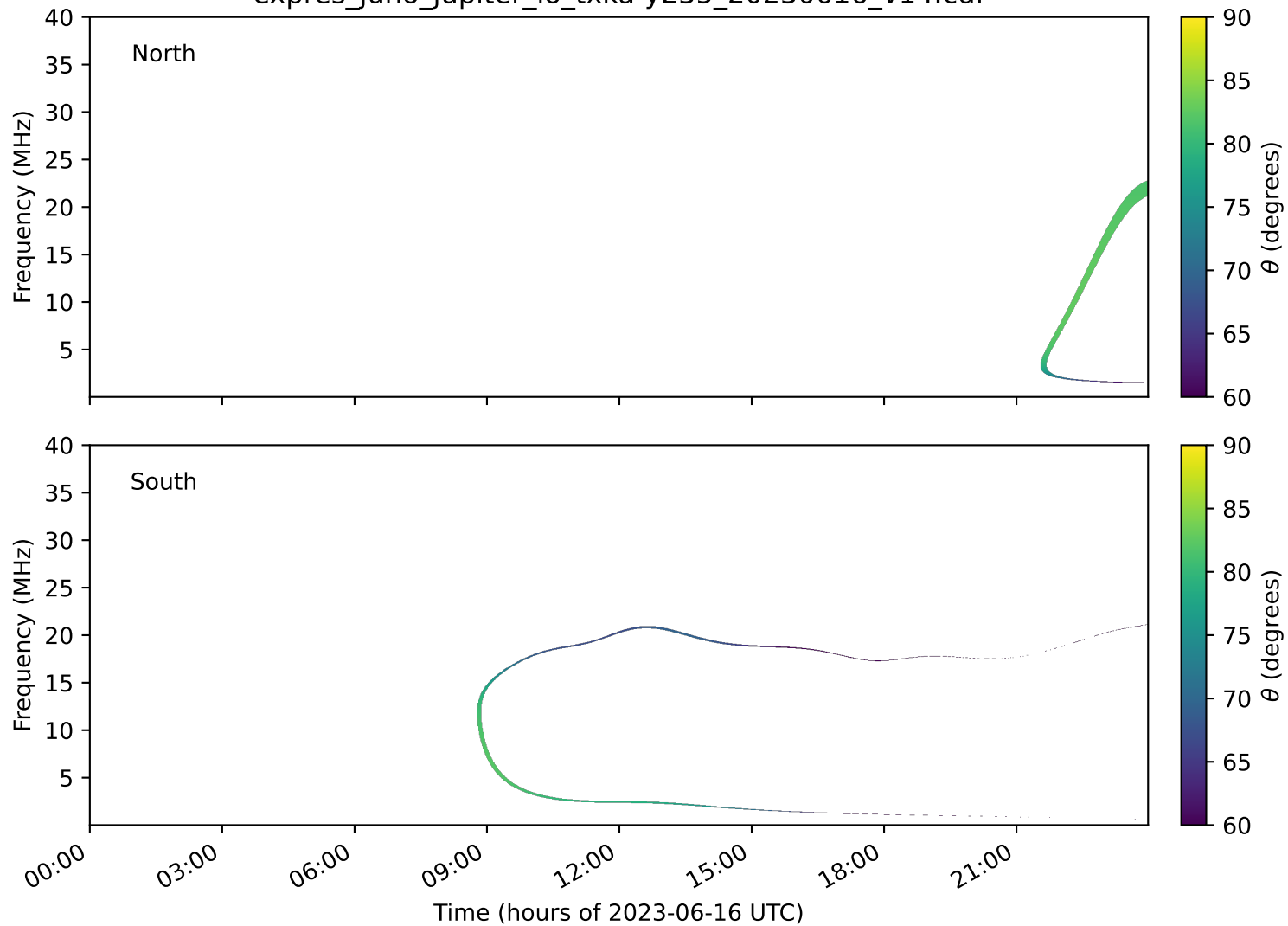
expres_juno_jupiter_io_txka-y235_20230616_v14.cdf
