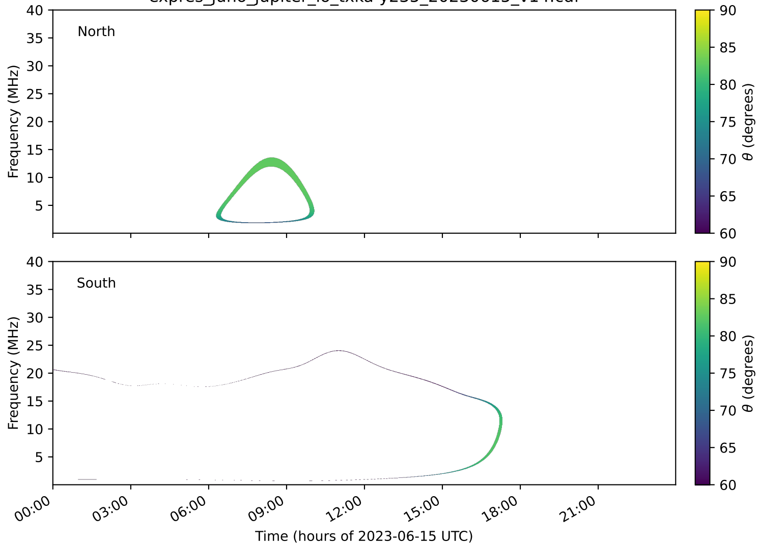
expres_juno_jupiter_io_txka-y235_20230615_v14.cdf
