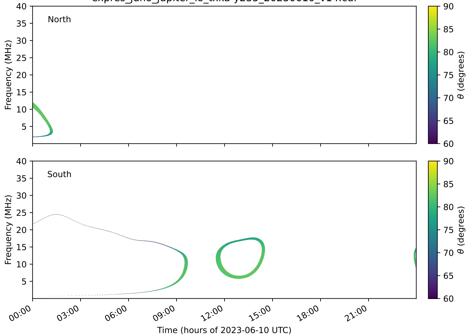
expres_juno_jupiter_io_txka-y235_20230610_v14.cdf
