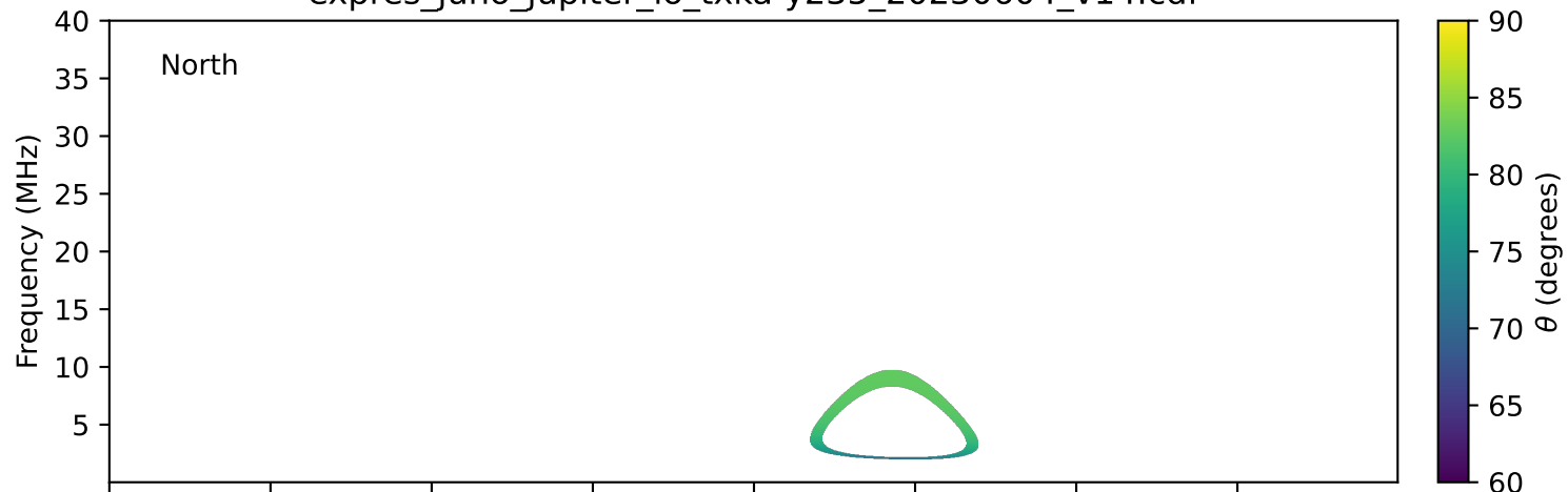
expres_juno_jupiter_io_txka-y235_20230604_v14.cdf
