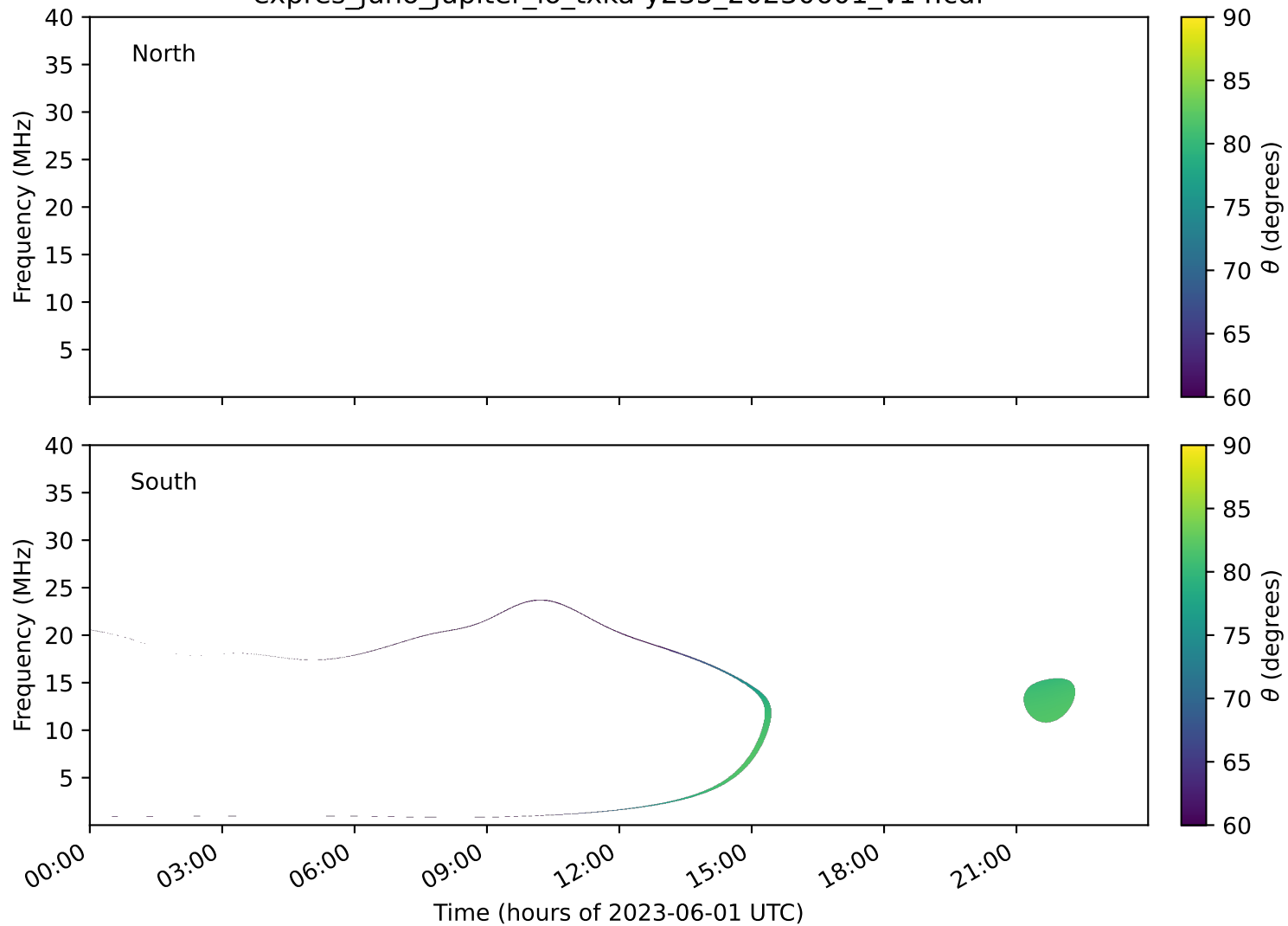
expres_juno_jupiter_io_txka-y235_20230601_v14.cdf
