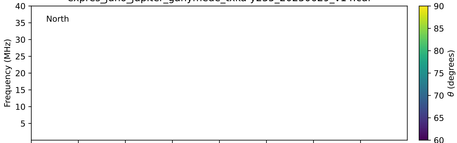
expres_juno_jupiter_ganymede_txka-y235_20230629_v14.cdf
