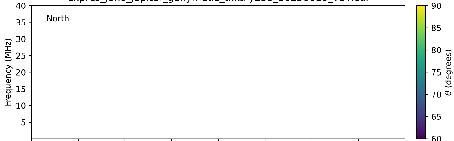
expres_juno_jupiter_ganymede_txka-y235_20230618_v14.cdf
