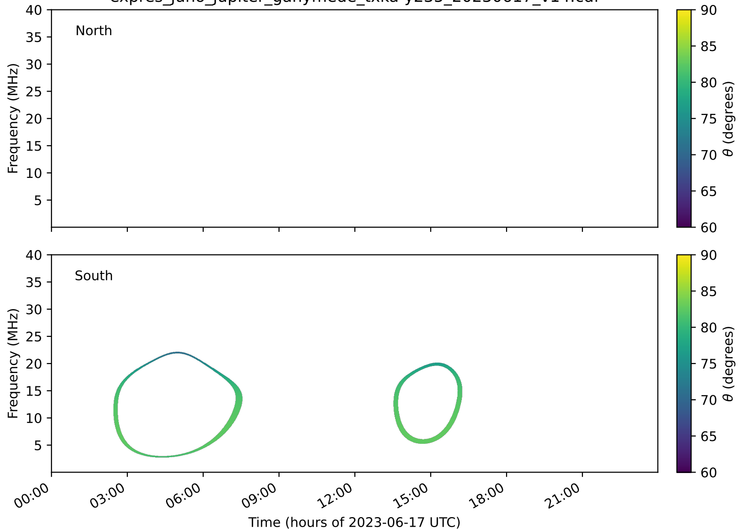
expres_juno_jupiter_ganymede_txka-y235_20230617_v14.cdf
