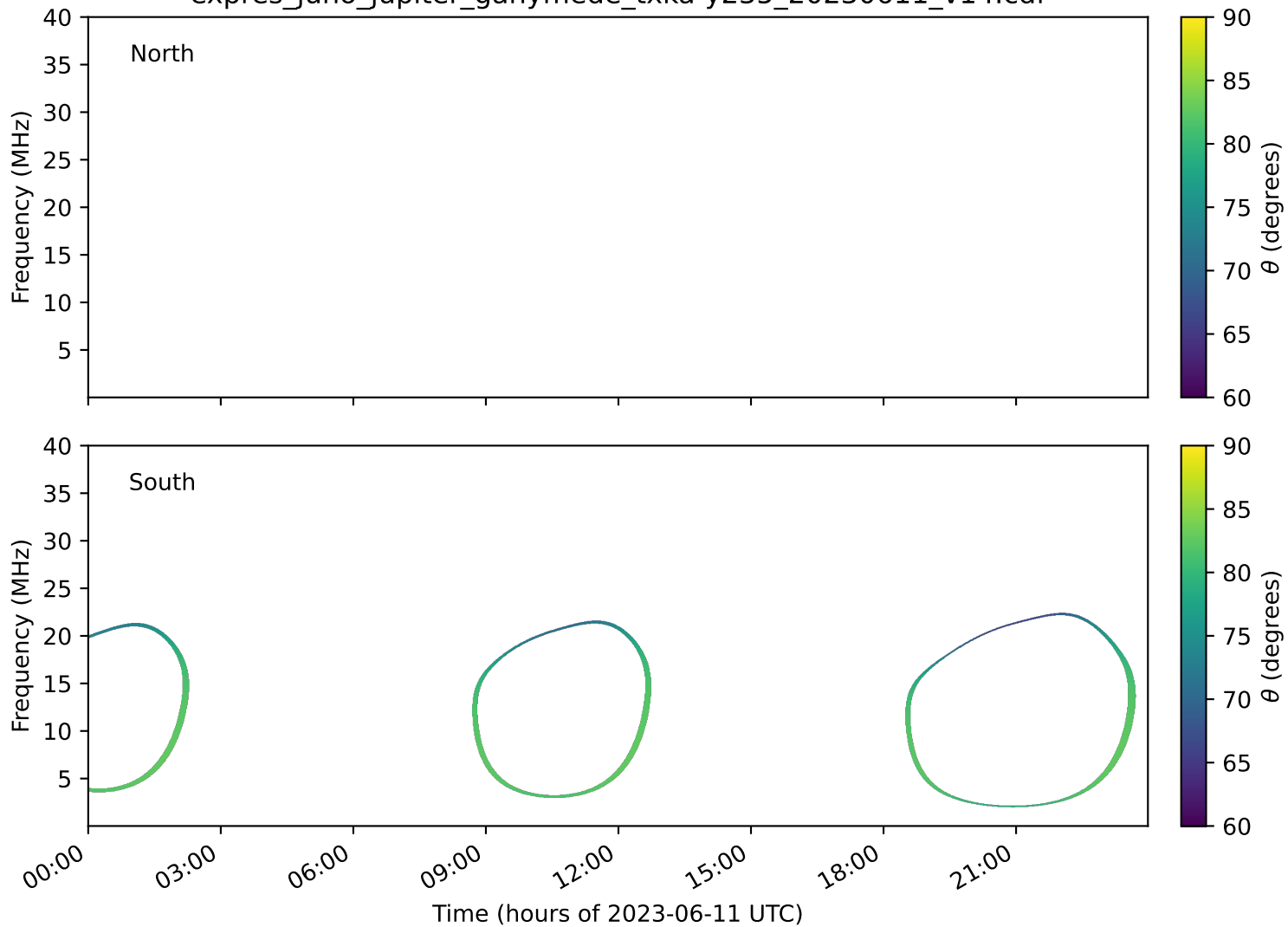
expres_juno_jupiter_ganymede_txka-y235_20230611_v14.cdf
