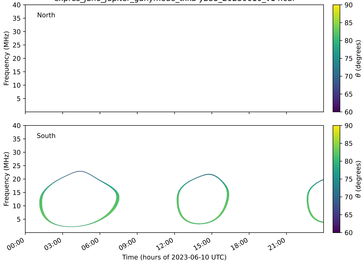
expres_juno_jupiter_ganymede_txka-y235_20230610_v14.cdf
