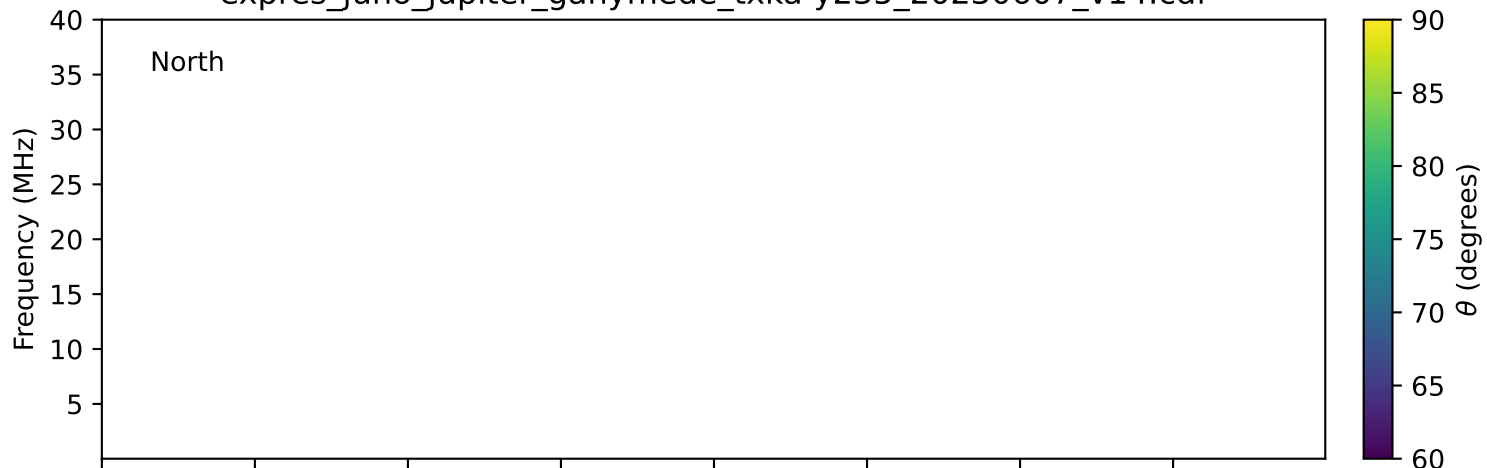
expres_juno_jupiter_ganymede_txka-y235_20230607_v14.cdf
