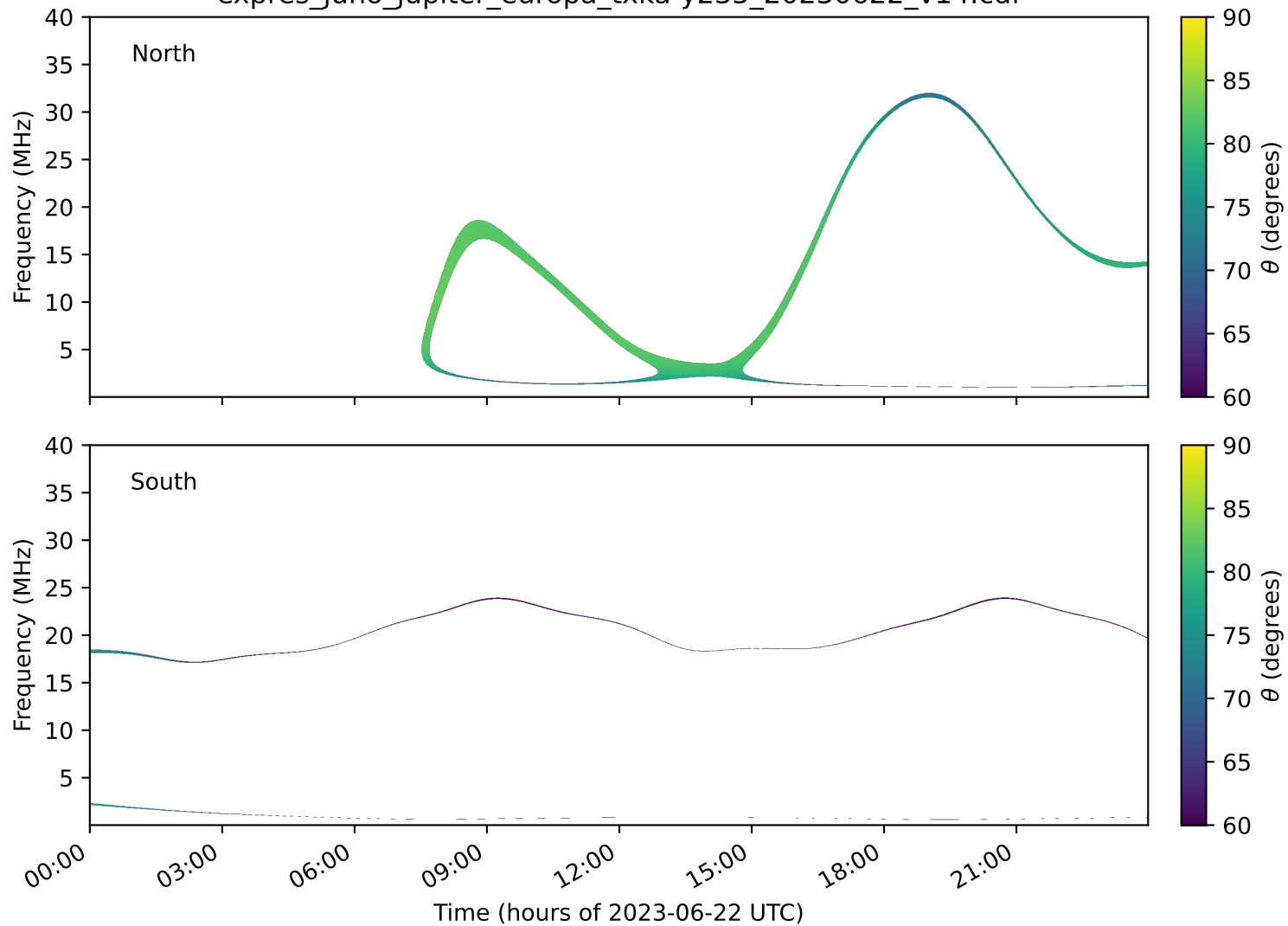
expres_juno_jupiter_europa_txka-y235_20230622_v14.cdf
