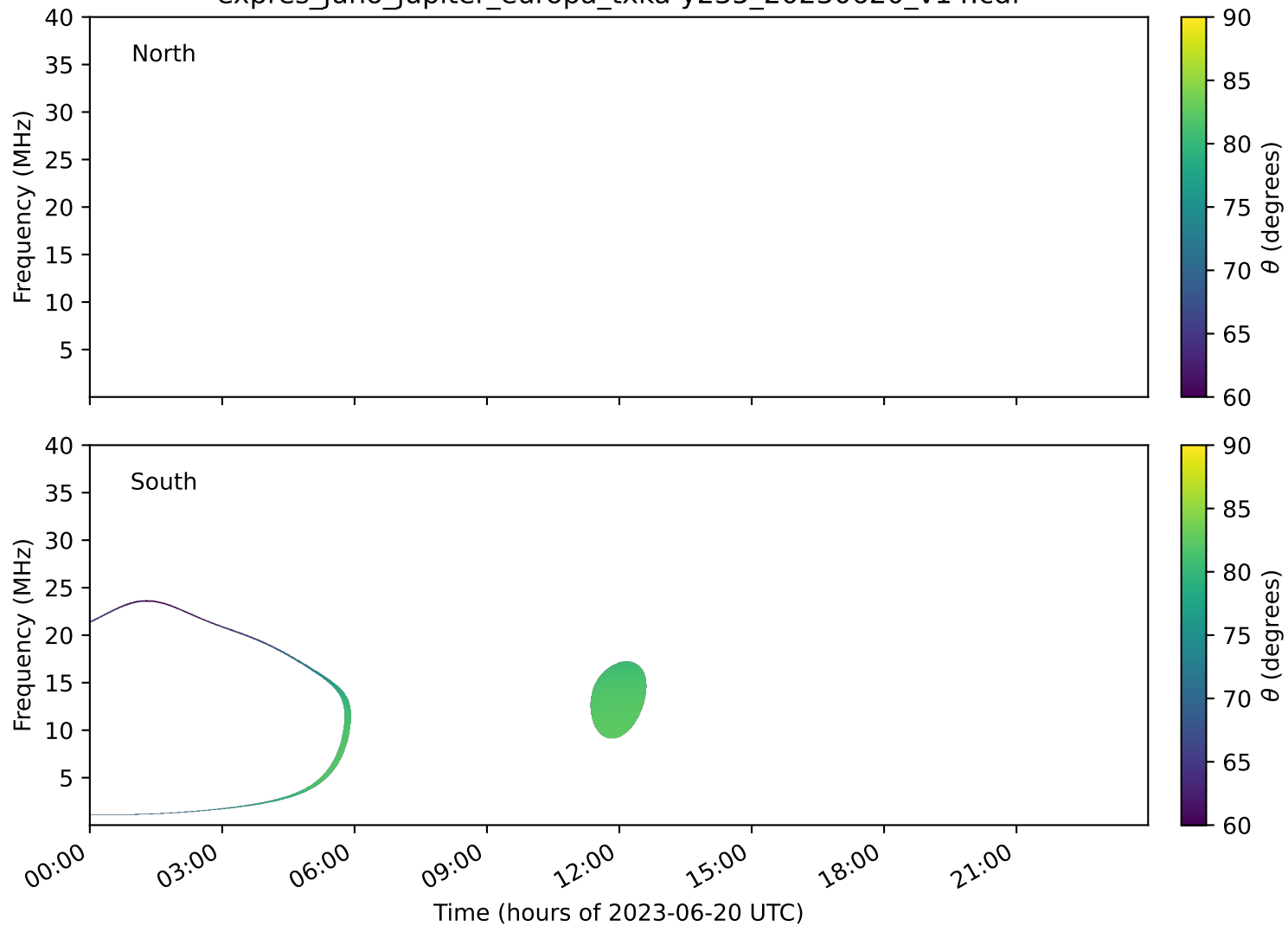
expres_juno_jupiter_europa_txka-y235_20230620_v14.cdf
