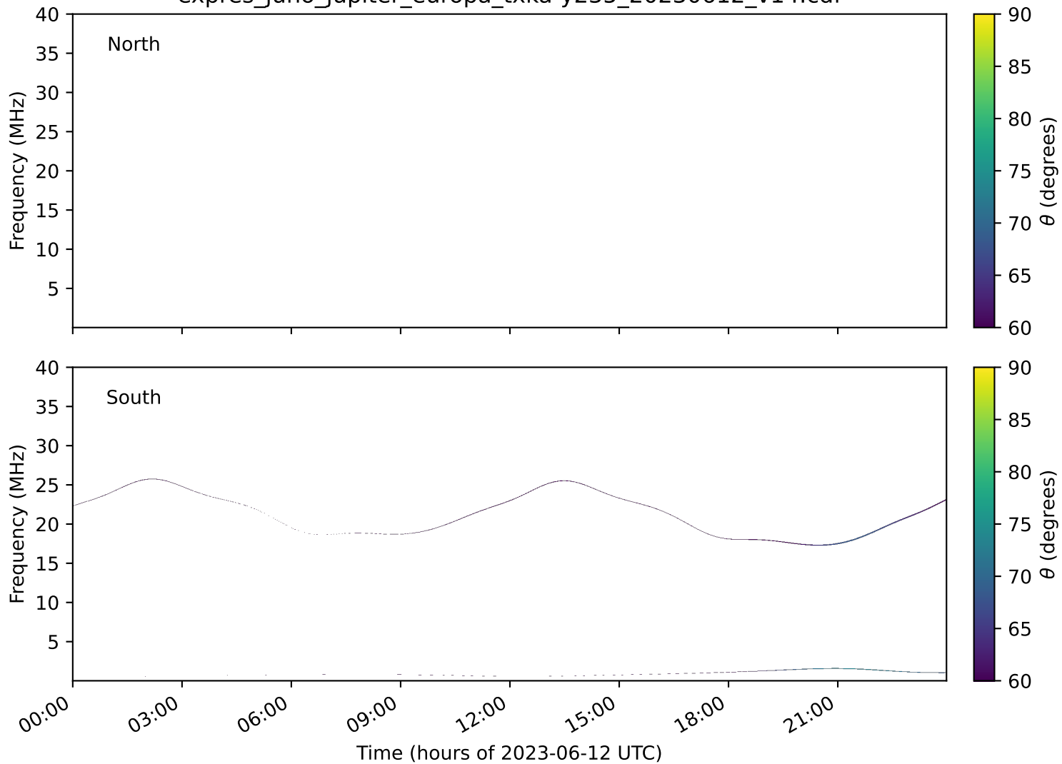
expres_juno_jupiter_europa_txka-y235_20230612_v14.cdf
