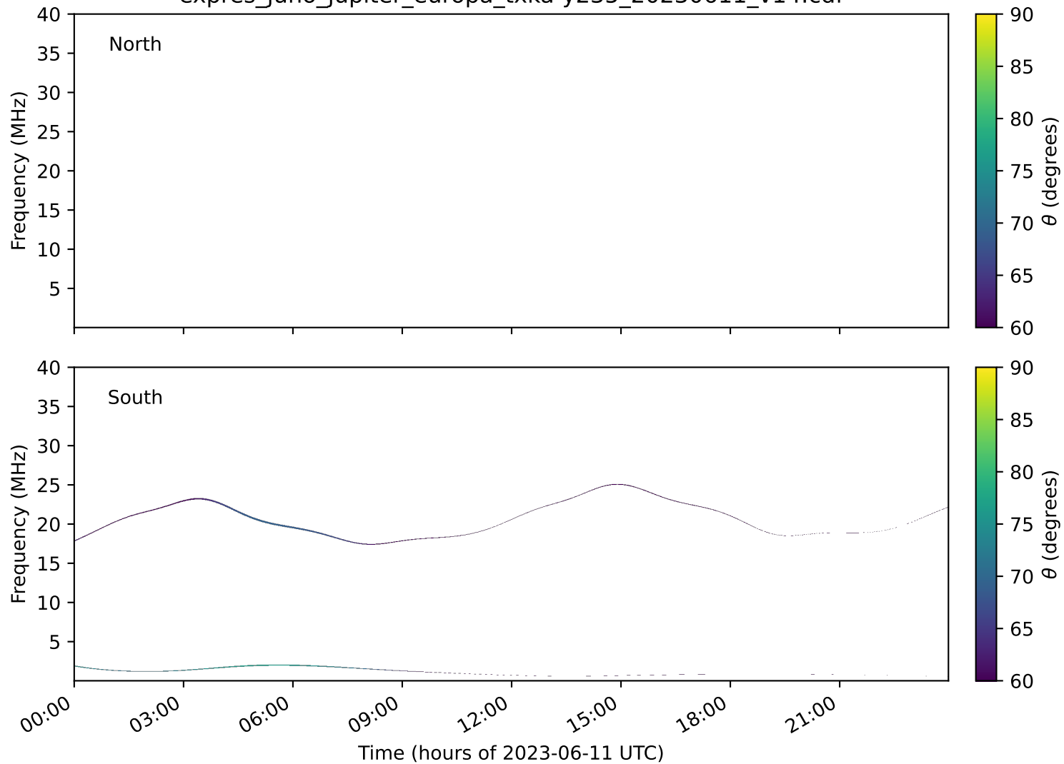
expres_juno_jupiter_europa_txka-y235_20230611_v14.cdf
