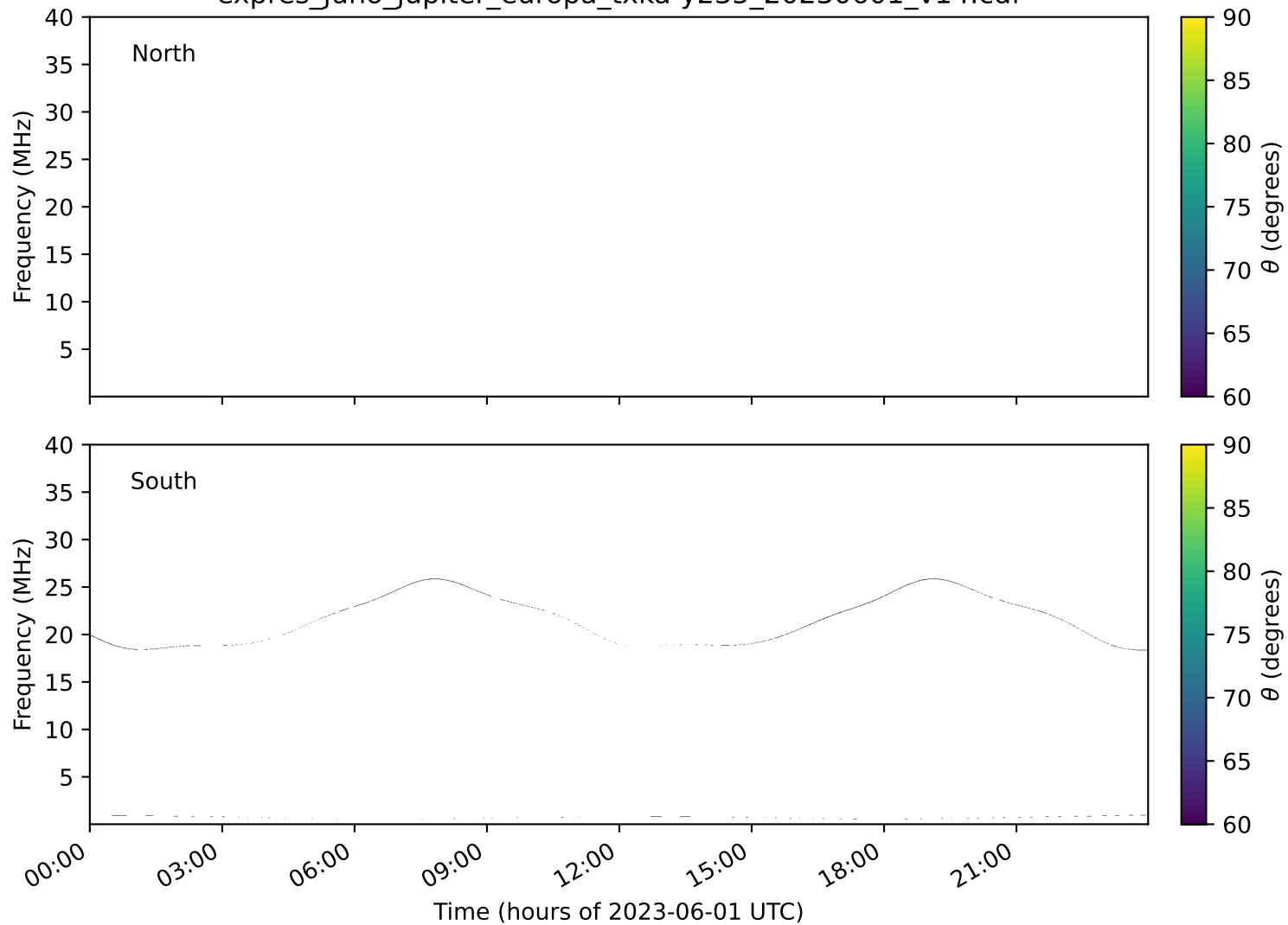
expres_juno_jupiter_europa_txka-y235_20230601_v14.cdf
