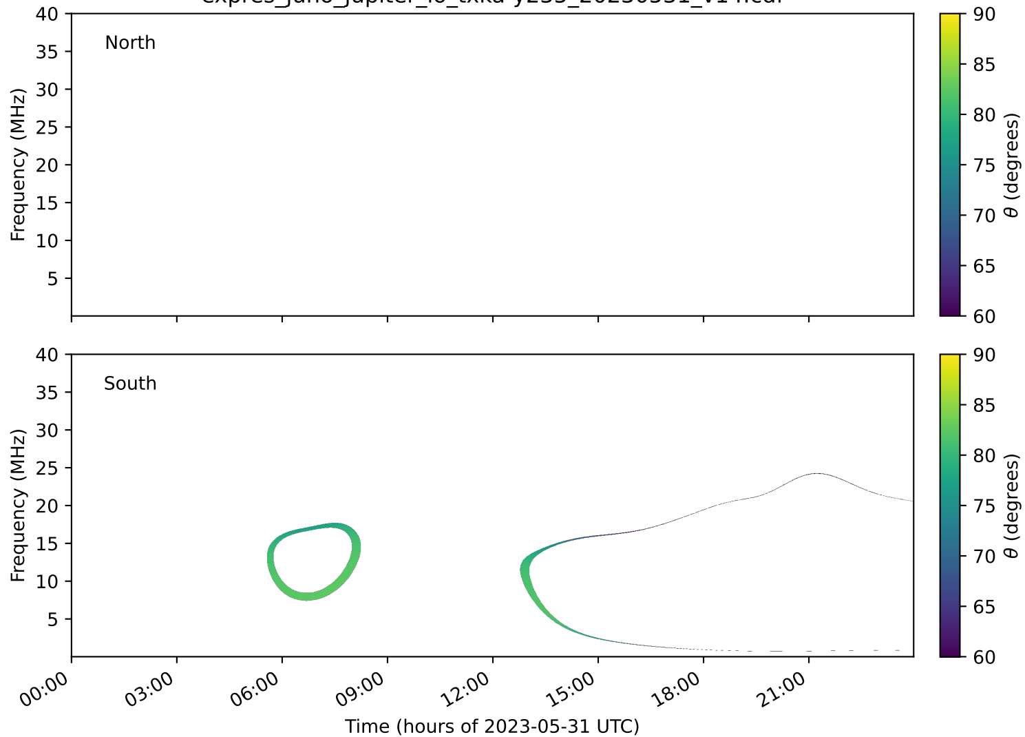
expres_juno_jupiter_io_txka-y235_20230531_v14.cdf
