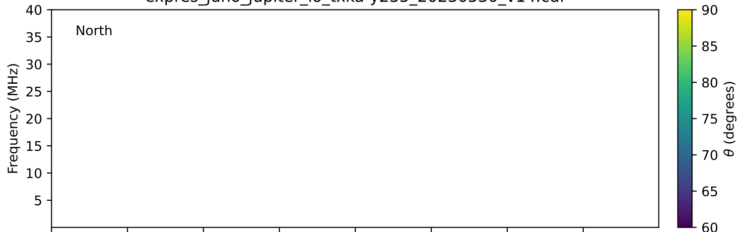
expres_juno_jupiter_io_txka-y235_20230530_v14.cdf
