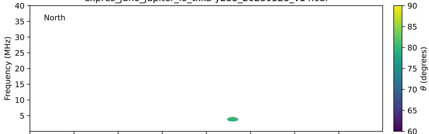
expres_juno_jupiter_io_txka-y235_20230528_v14.cdf
