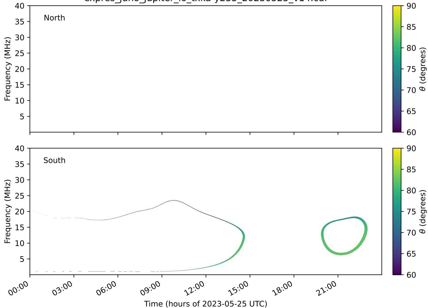
expres_juno_jupiter_io_txka-y235_20230525_v14.cdf
