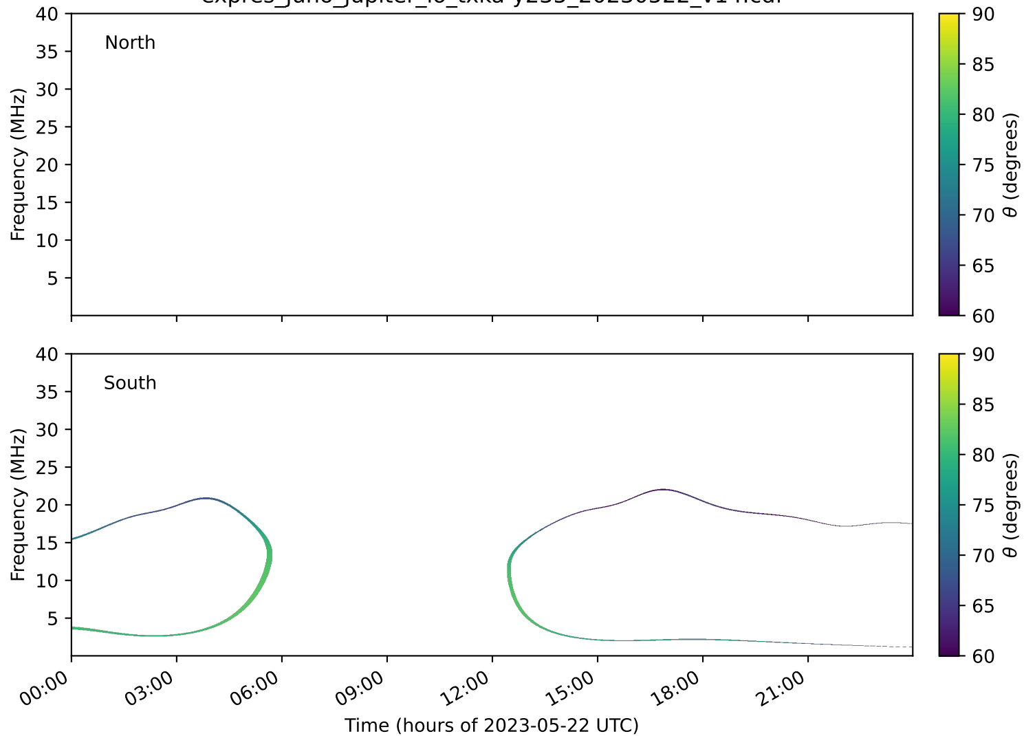
expres_juno_jupiter_io_txka-y235_20230522_v14.cdf
