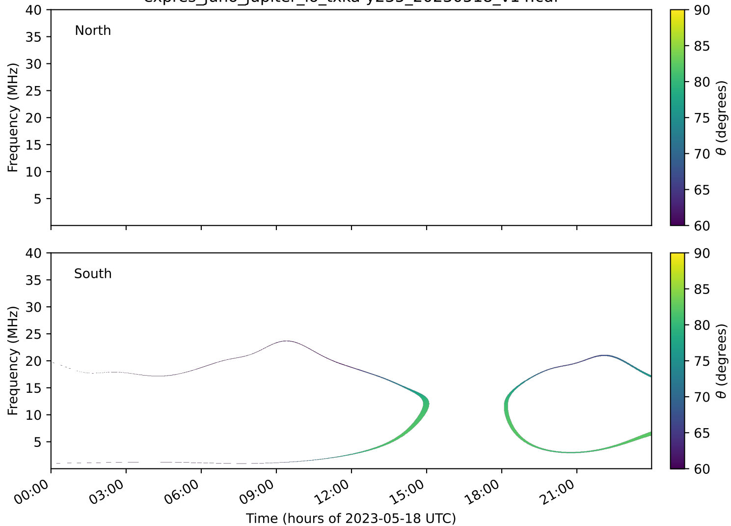
expres_juno_jupiter_io_txka-y235_20230518_v14.cdf
