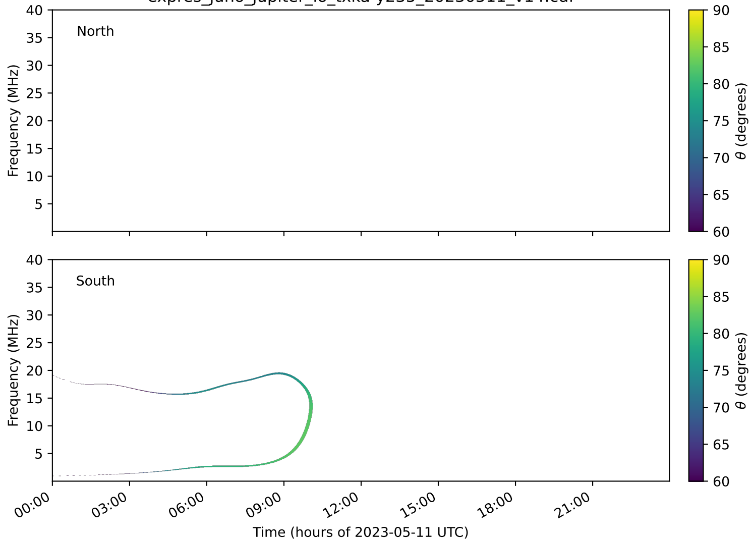
expres_juno_jupiter_io_txka-y235_20230511_v14.cdf
