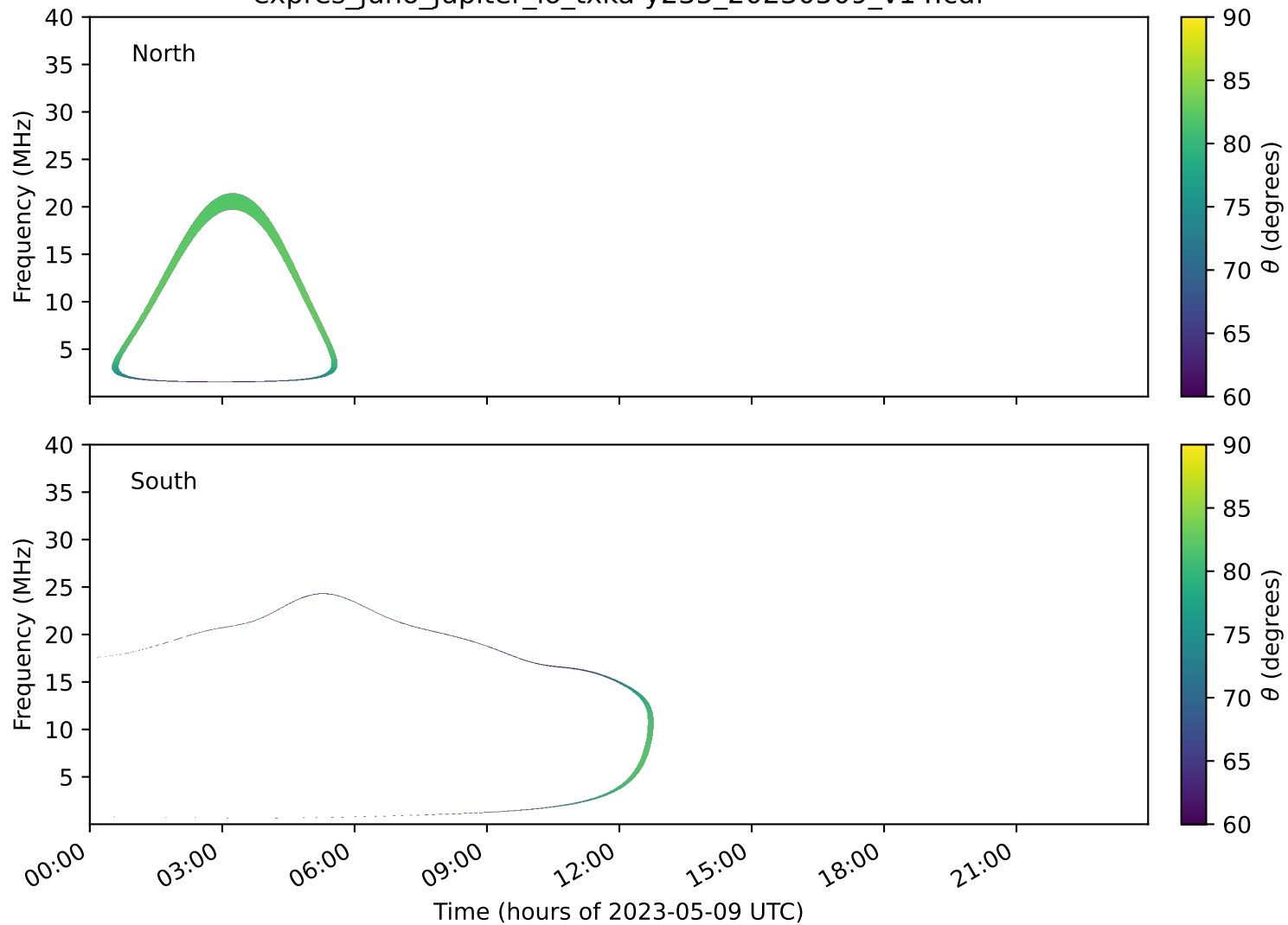
expres_juno_jupiter_io_txka-y235_20230509_v14.cdf
