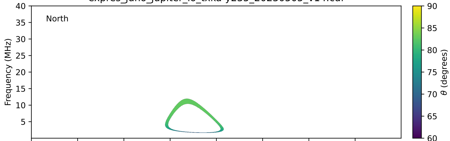
expres_juno_jupiter_io_txka-y235_20230505_v14.cdf
