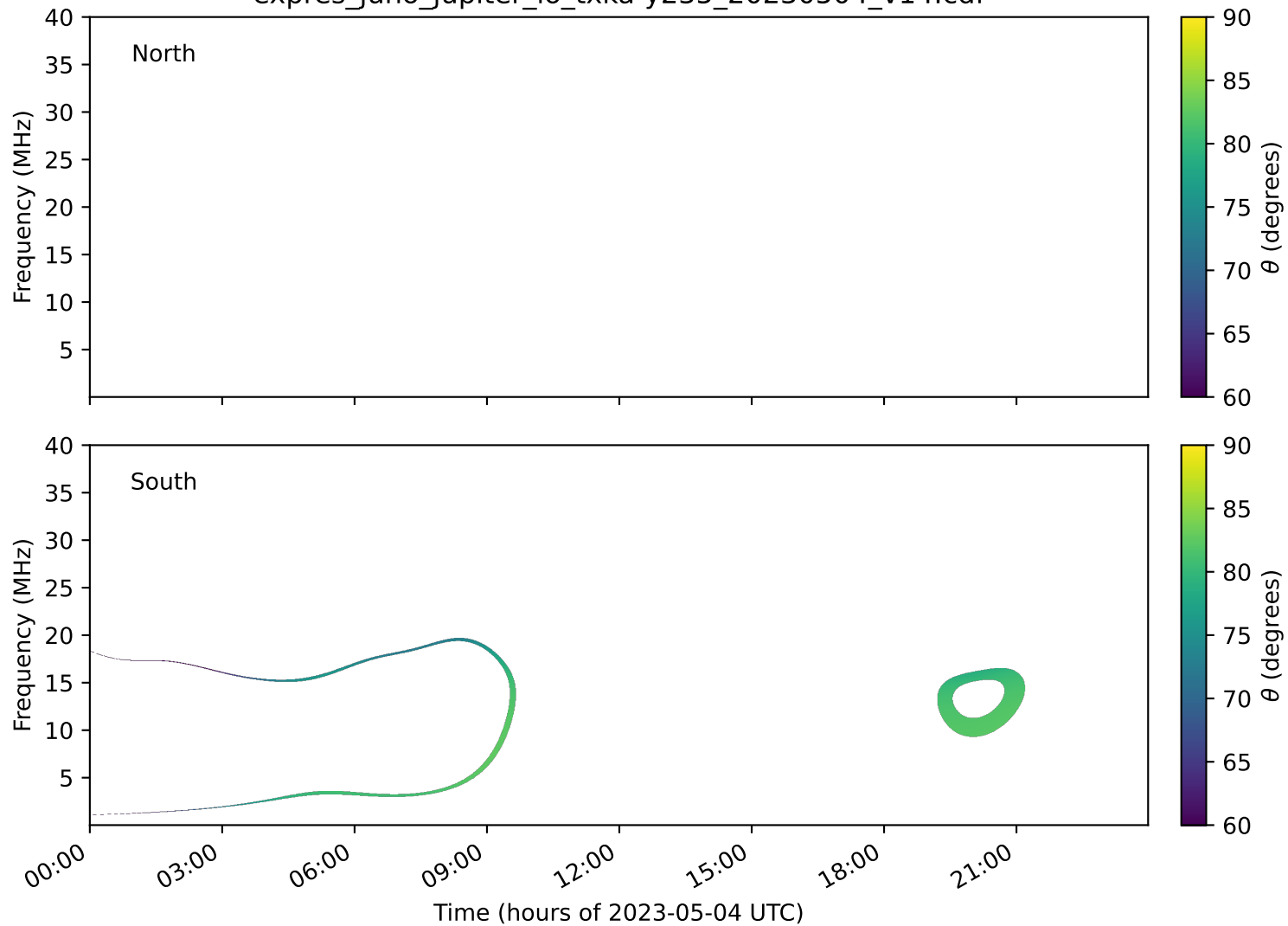
expres_juno_jupiter_io_txka-y235_20230504_v14.cdf
