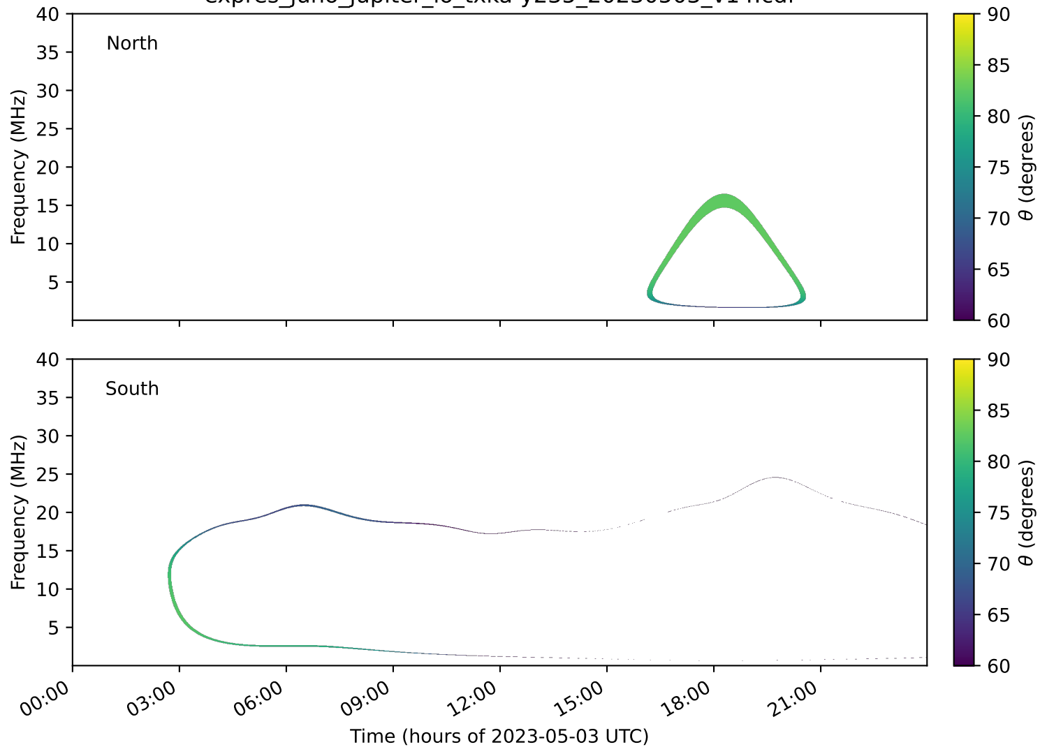
expres_juno_jupiter_io_txka-y235_20230503_v14.cdf
