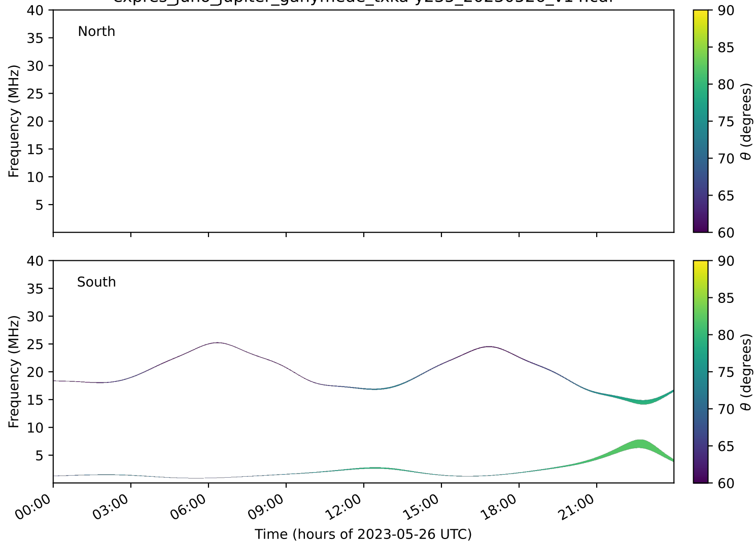
expres_juno_jupiter_ganymede_txka-y235_20230526_v14.cdf
