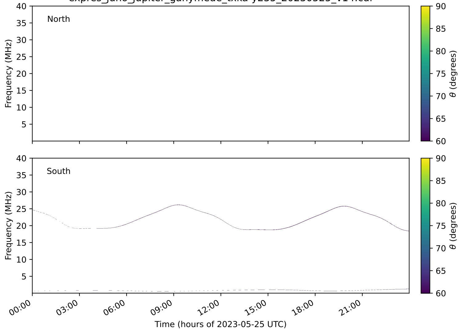
expres_juno_jupiter_ganymede_txka-y235_20230525_v14.cdf
