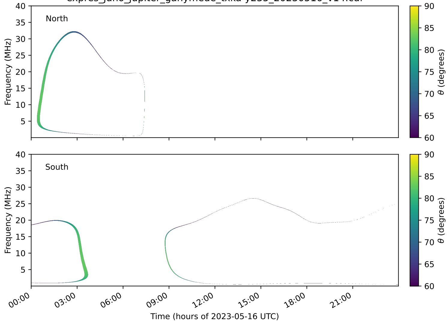
expres_juno_jupiter_ganymede_txka-y235_20230516_v14.cdf
