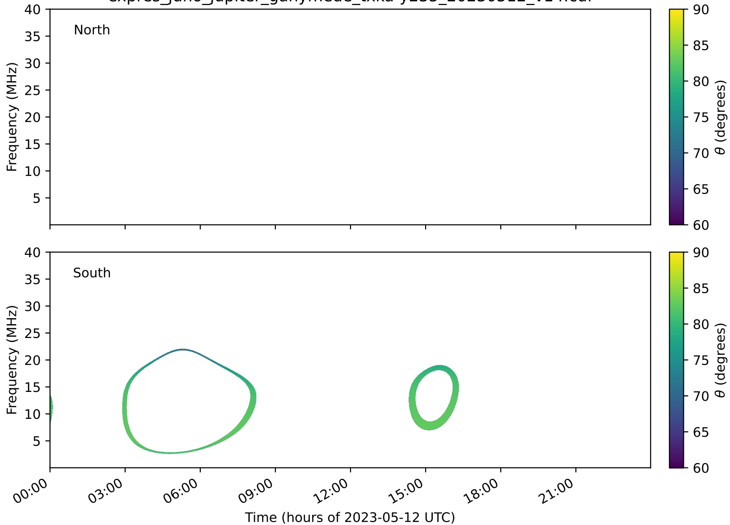
expres_juno_jupiter_ganymede_txka-y235_20230512_v14.cdf
