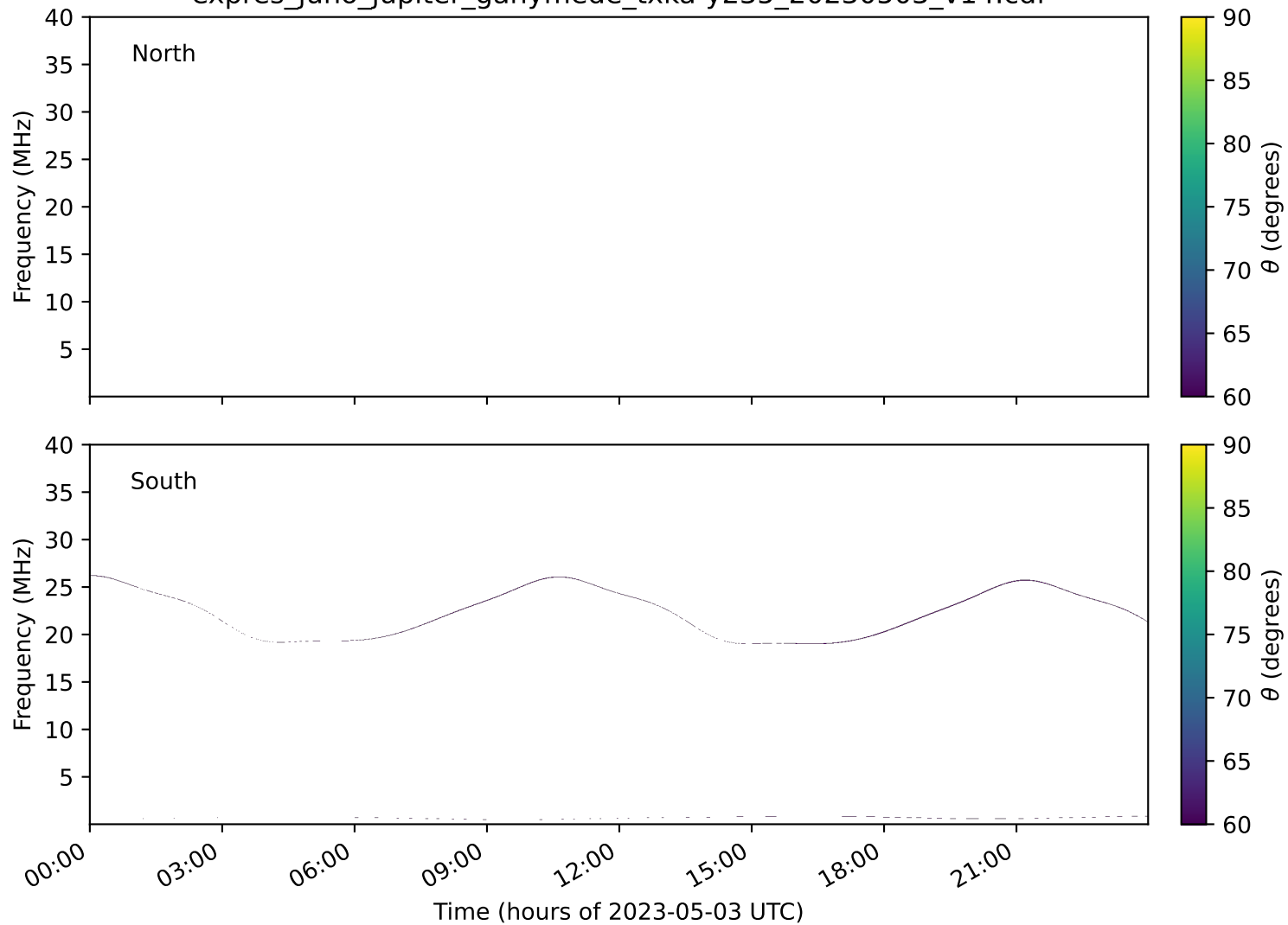
expres_juno_jupiter_ganymede_txka-y235_20230503_v14.cdf
