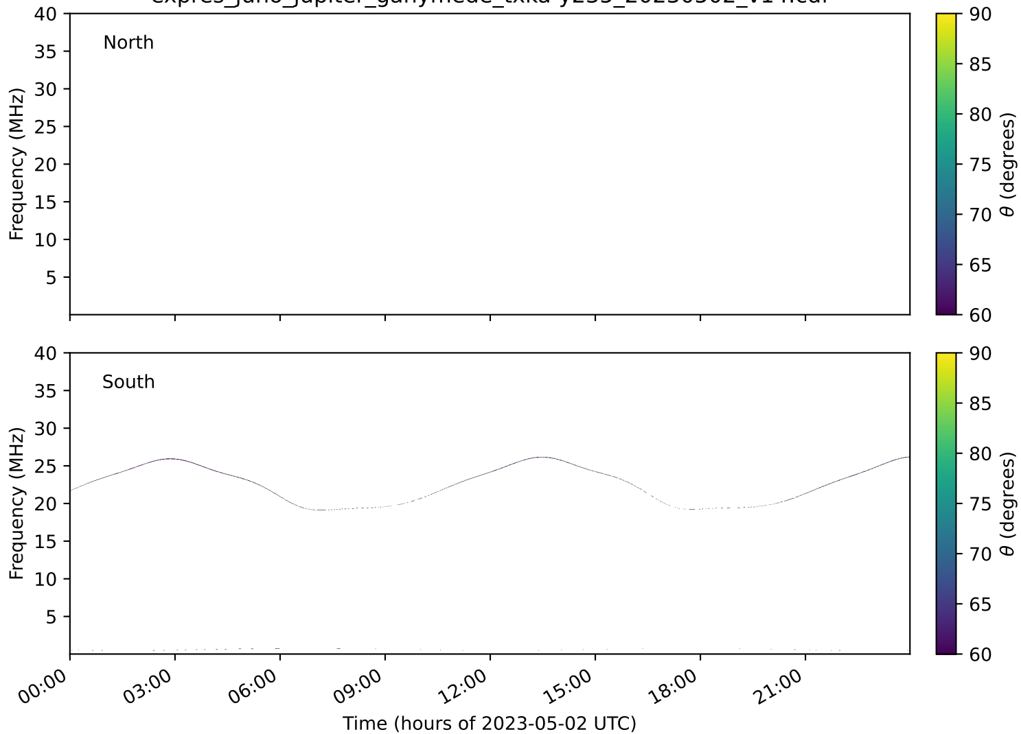
expres_juno_jupiter_ganymede_txka-y235_20230502_v14.cdf
