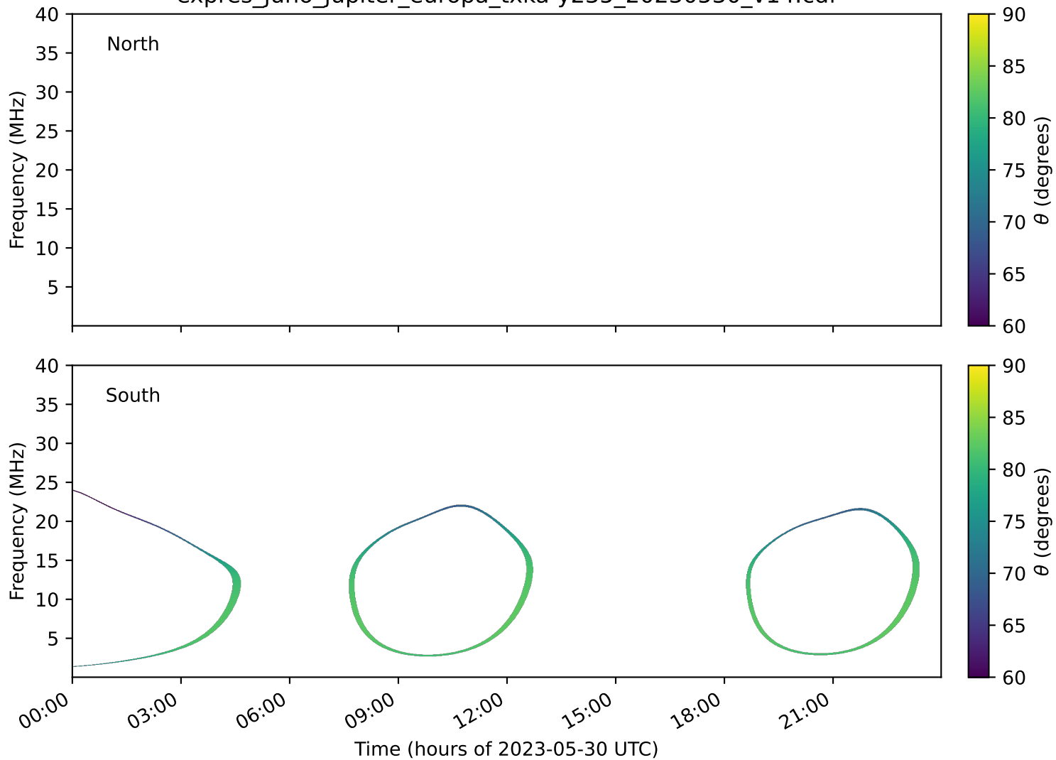
expres_juno_jupiter_europa_txka-y235_20230530_v14.cdf
