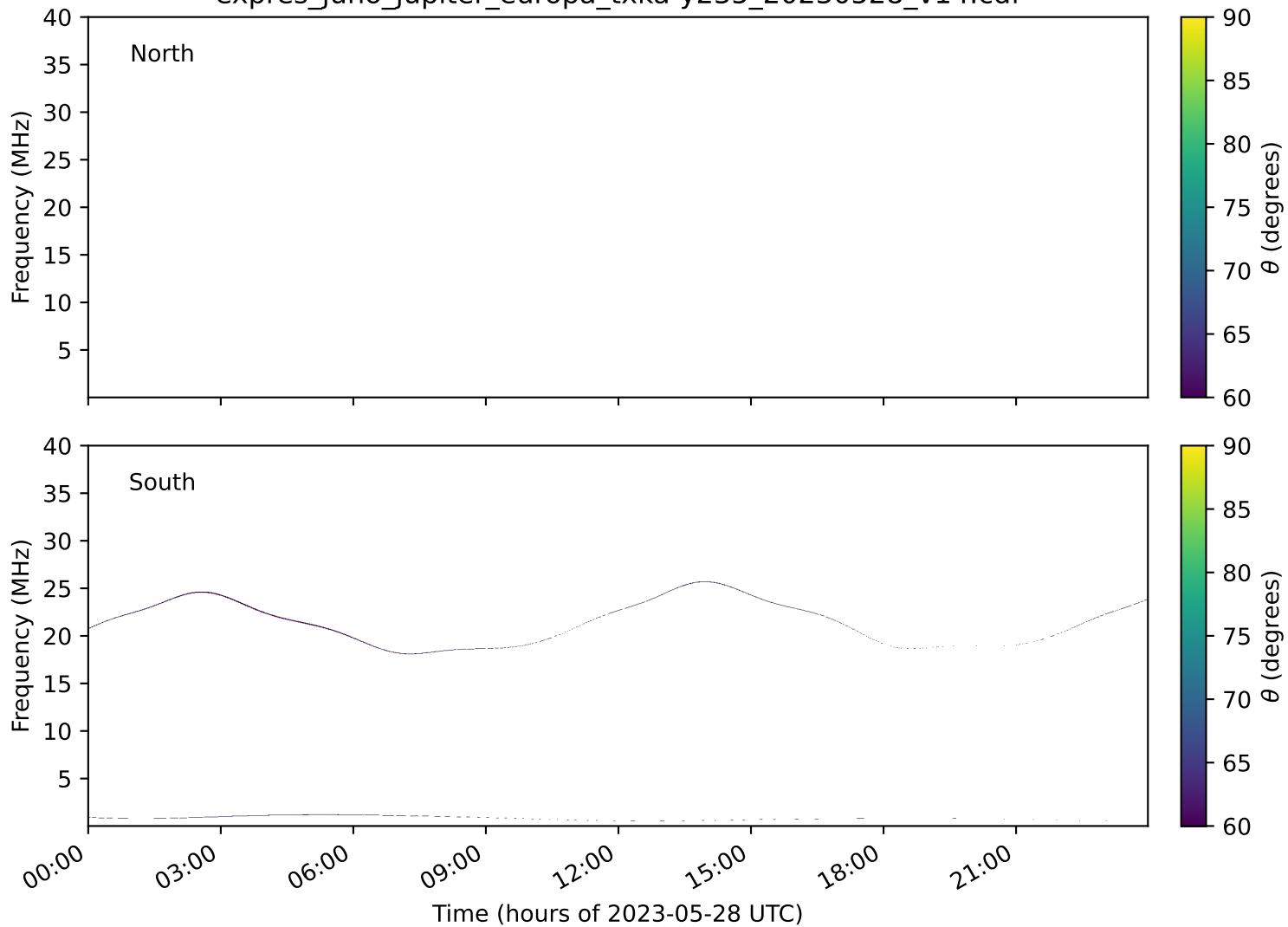
expres_juno_jupiter_europa_txka-y235_20230528_v14.cdf
