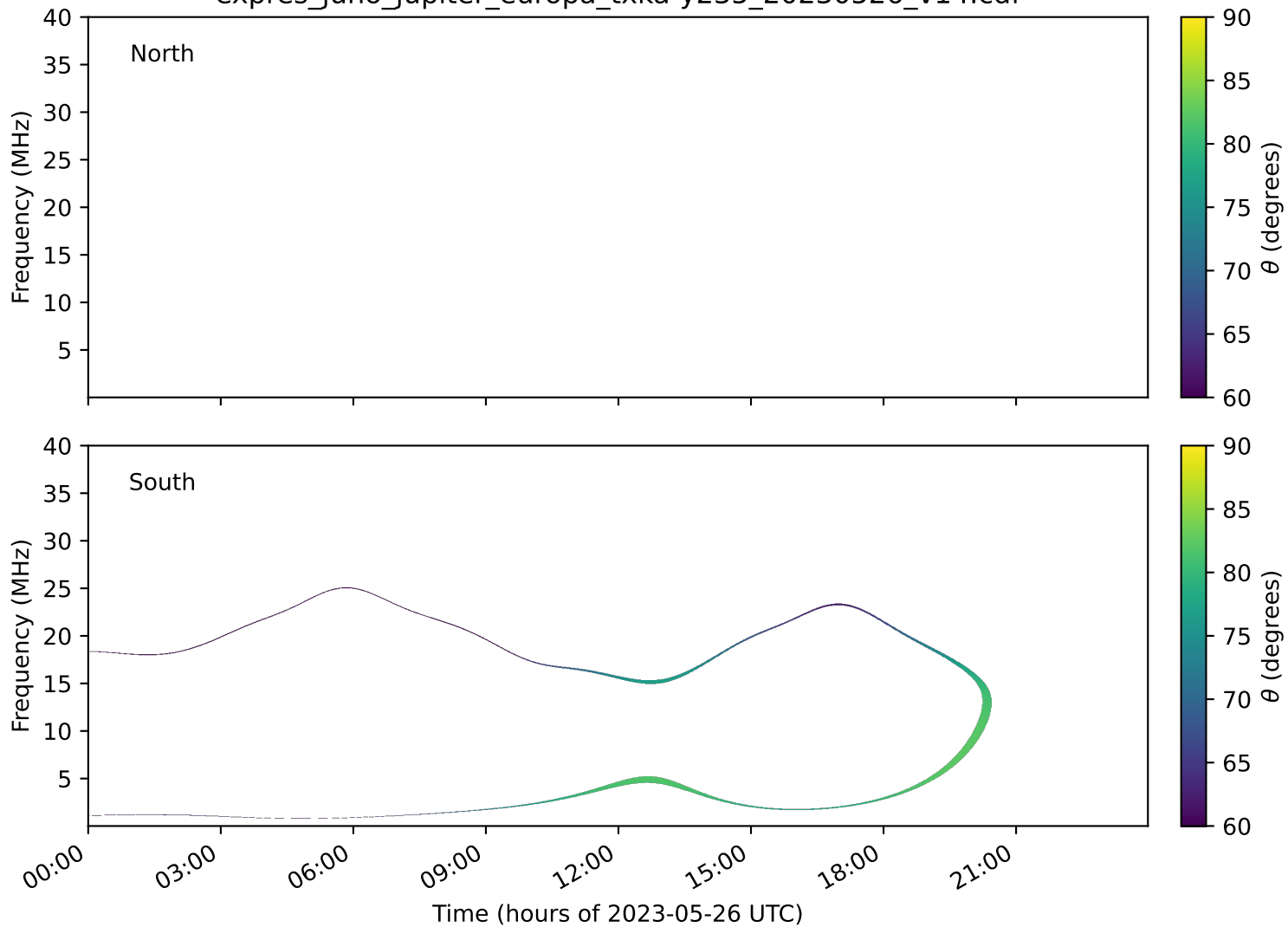
expres_juno_jupiter_europa_txka-y235_20230526_v14.cdf
