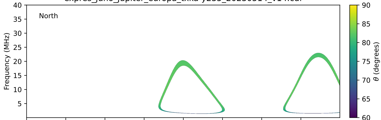
expres_juno_jupiter_europa_txka-y235_20230514_v14.cdf
