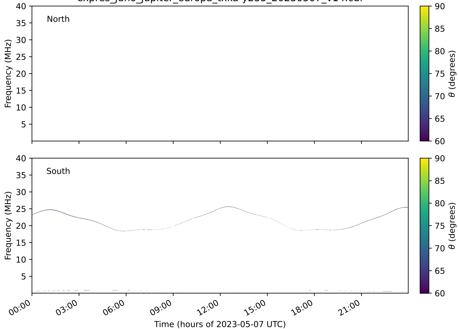
expres_juno_jupiter_europa_txka-y235_20230507_v14.cdf
