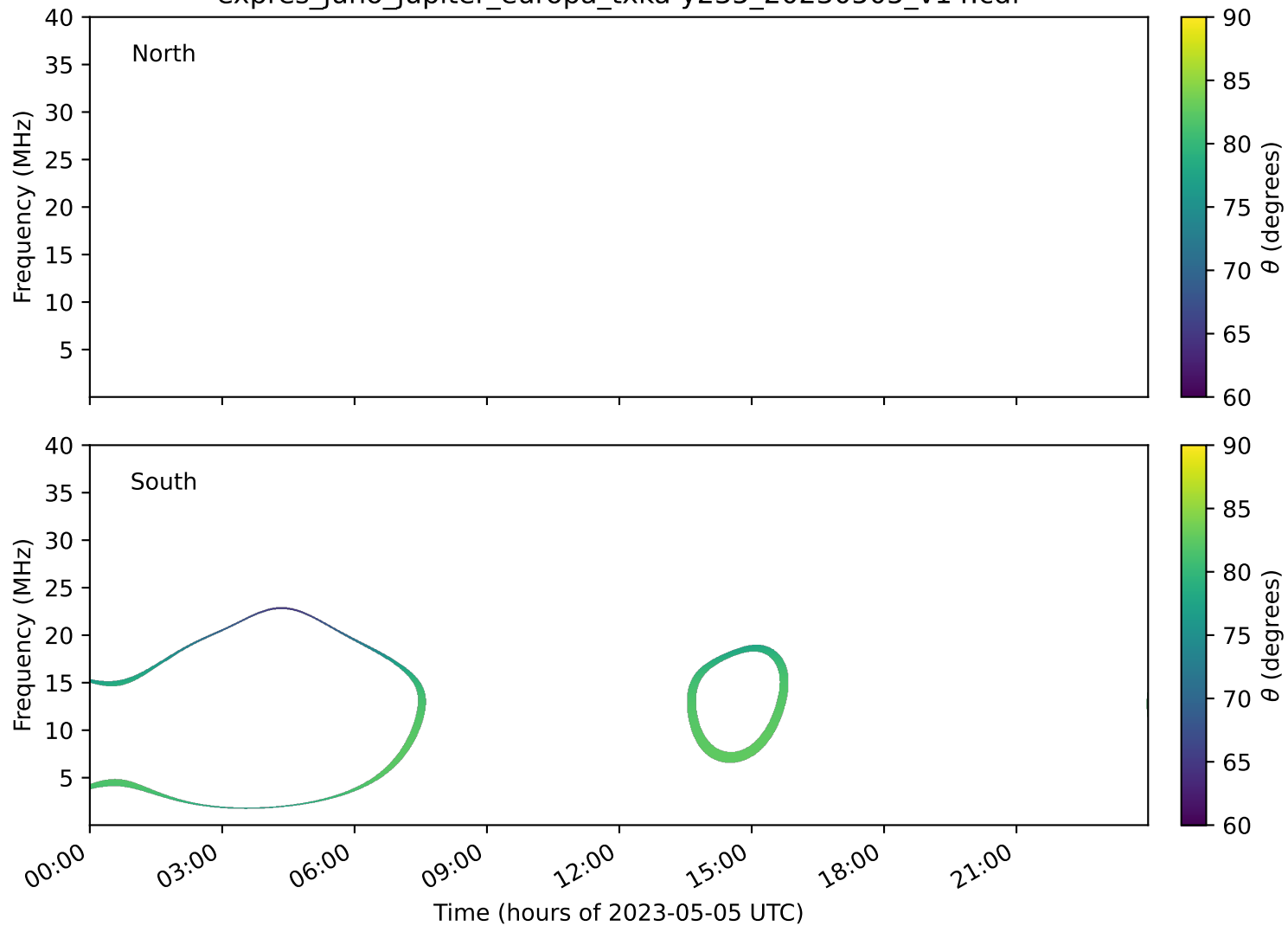
expres_juno_jupiter_europa_txka-y235_20230505_v14.cdf
