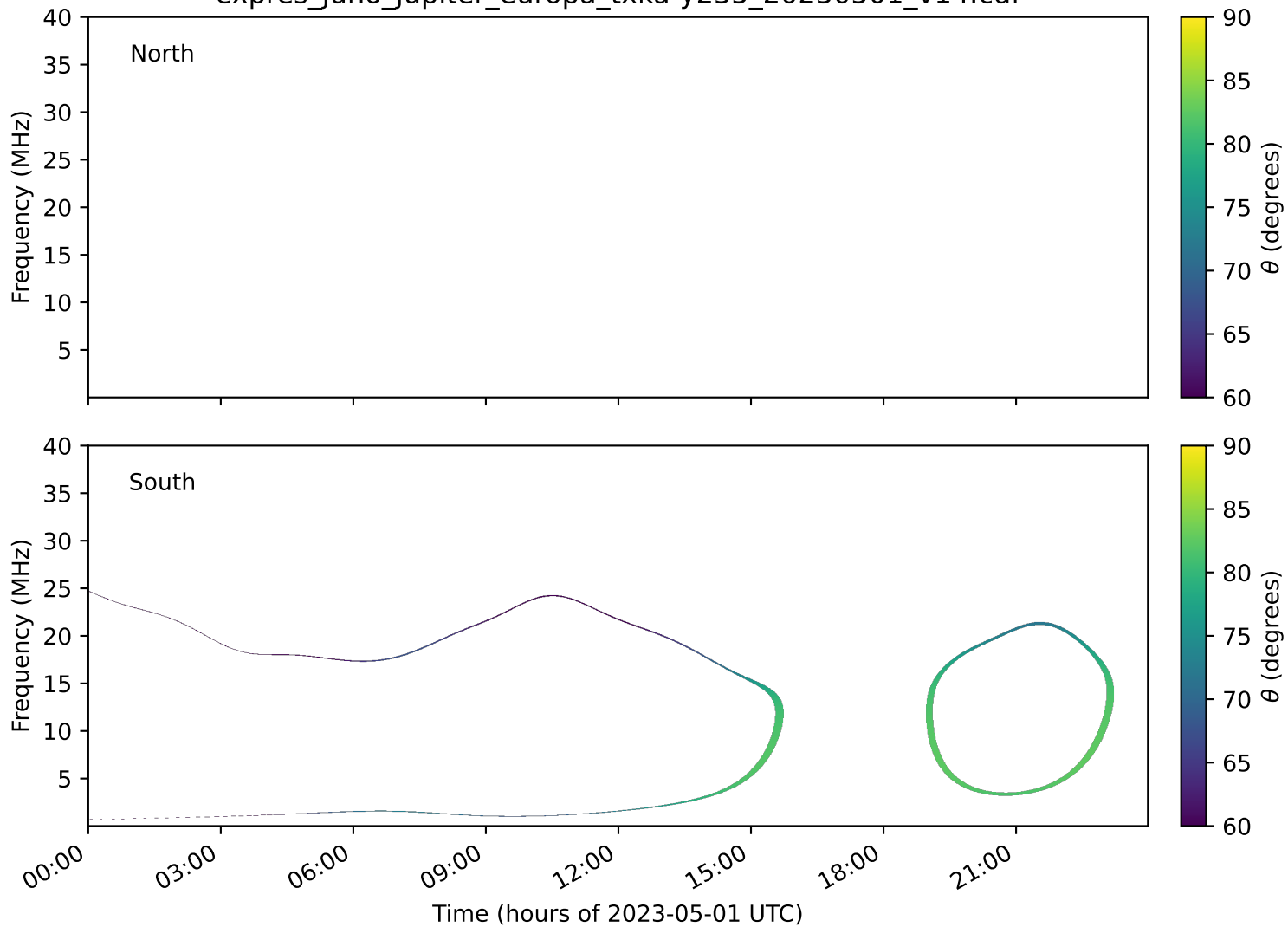
expres_juno_jupiter_europa_txka-y235_20230501_v14.cdf
