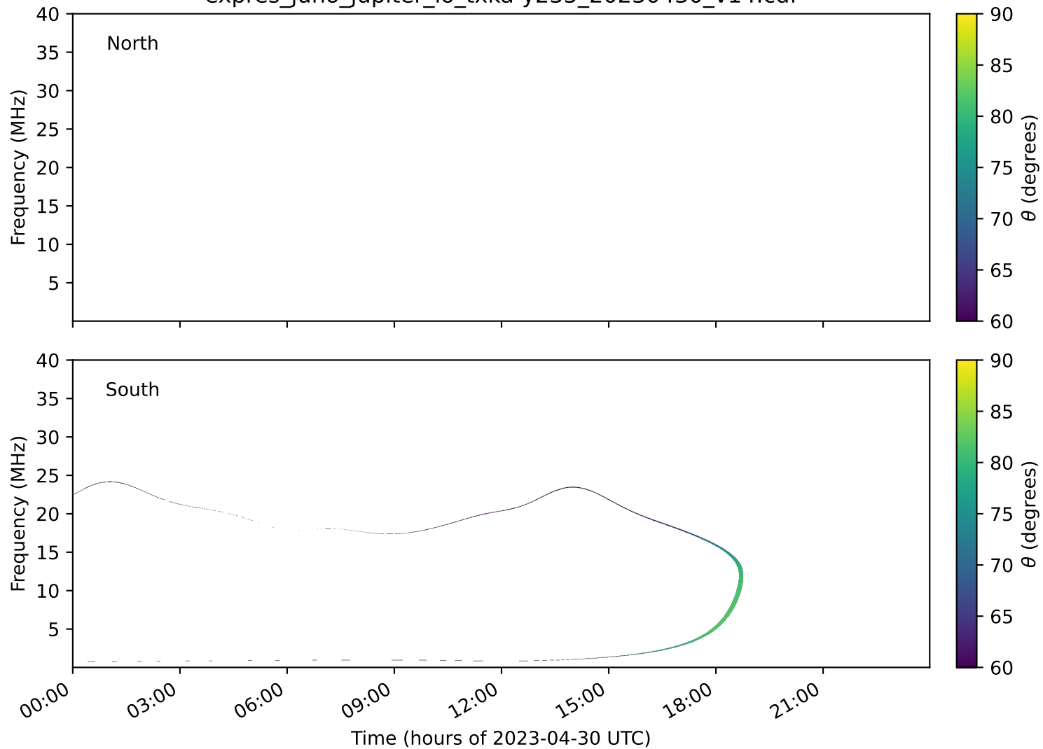
expres_juno_jupiter_io_txka-y235_20230430_v14.cdf
