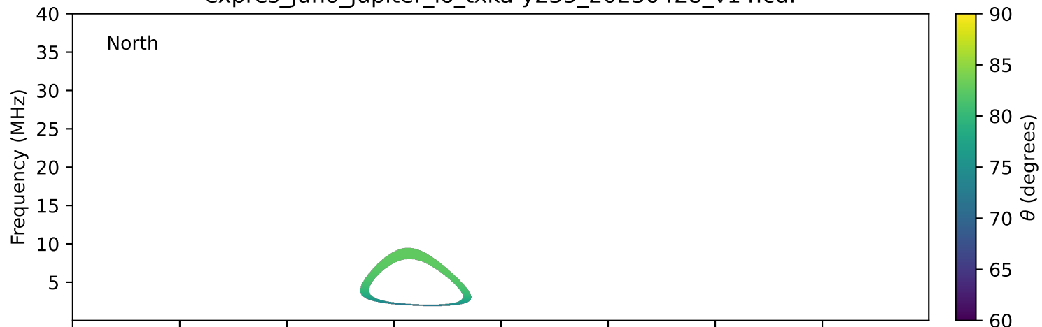
expres_juno_jupiter_io_txka-y235_20230428_v14.cdf
