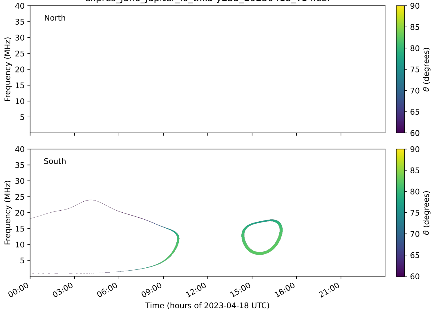
expres_juno_jupiter_io_txka-y235_20230418_v14.cdf
